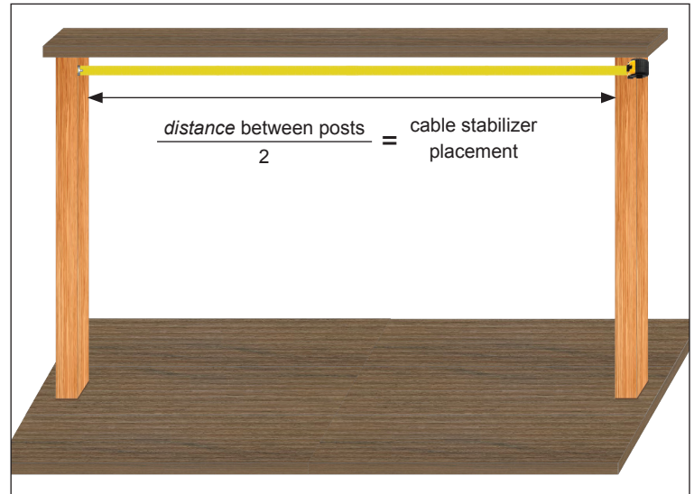
Figure A. Calculate horizontal distance between posts and divide by two.
