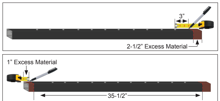
Figure D. (TOP) Using the measurement from Figure B, measure from the center of an outer hole toward the end of the stabilizer and mark.
