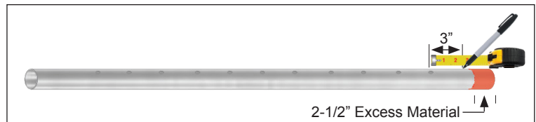
Figure AB. Using the measurement from Figure B, measure from the center of an outer hole toward the end of the stabilizer and mark.
