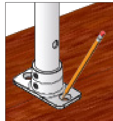
Figure AY. (LEFT) Mark screw holes in the cable stabilizer adjustable base with a pencil.
