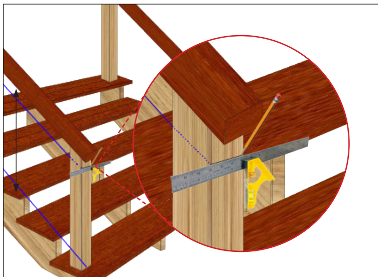
Figure AQ. Using a carpenter's square, transfer a line to the inside post face to find the center of your cable.
