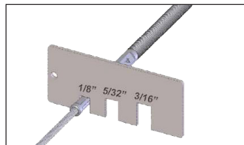
Figure D. Measure the fitting as shown after the first swage. Adjust the tool accordingly before completing any additional swaging.
